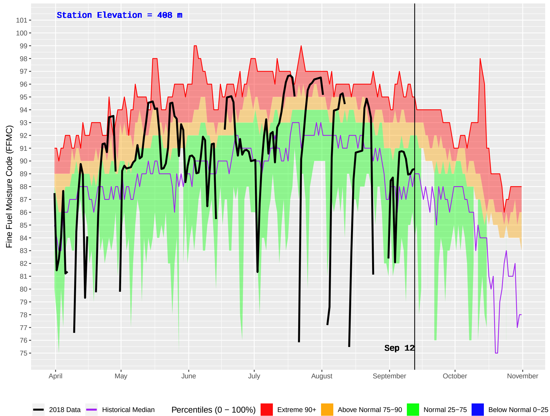
LILLOOET (280) : Historical (1977–2016) and Current (2018) Daily Fine Fuel Moisture Code (FFMC)
